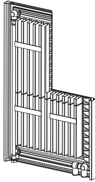
P5KV cutaway with convector fins, rear view
