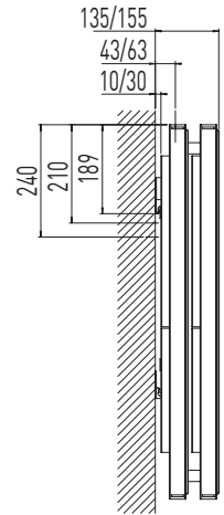
P5KV-D, profile
