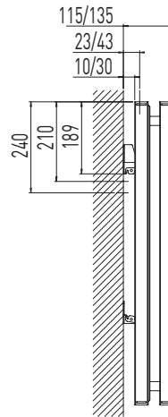
P5V-D, profile
