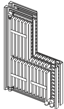
P5KV-D cutaway with convector fins, rear view
