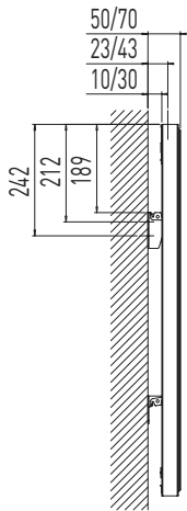
P5V, profile
