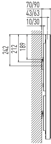
P5KV, profile
